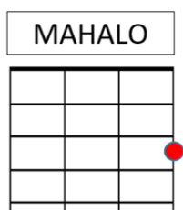
C major chord
