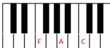
F major chord
