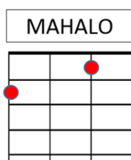
F major chord
